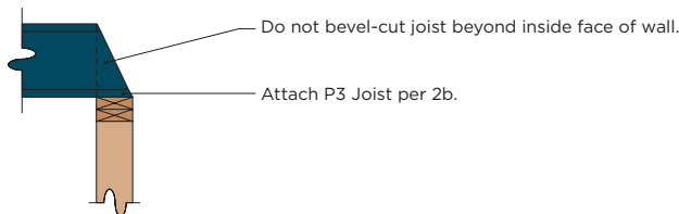
2n BEVEL-CUT P3 JOIST DETAIL
