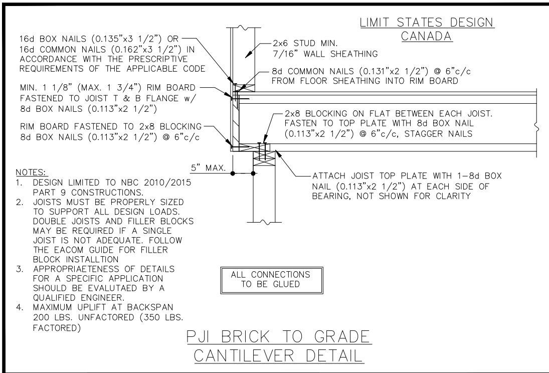
Figure 1: PJI Brick Cantilever Detail
