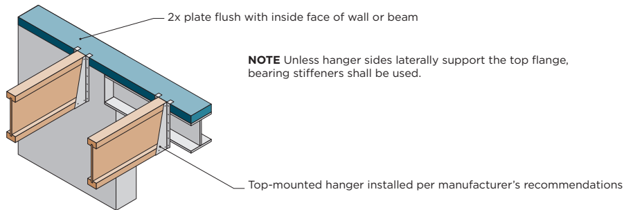
2k P3 JOIST WITH TOP MOUNT HANGER DETAIL
