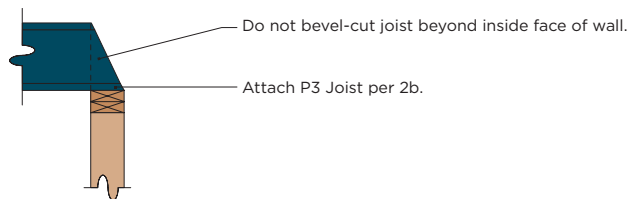
2n BEVEL-CUT P3 JOIST DETAIL
