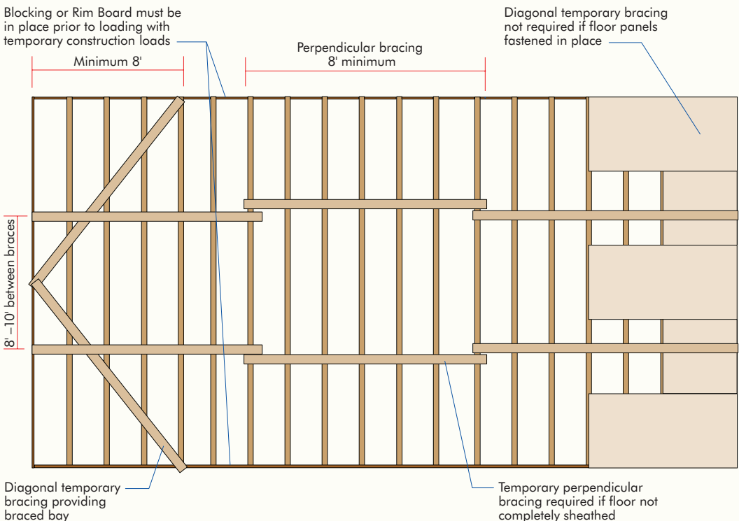
FIGURE 1 TEMPORARY CONSTRUCTION BRACING
