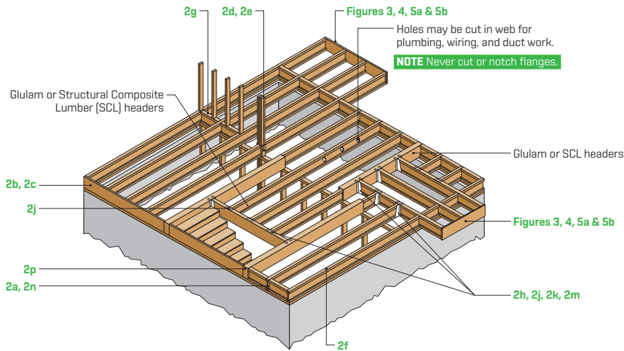
FIGURE 2 Typical P3 Floor Joist Framing and Construction Details
