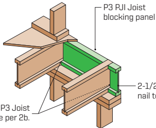
2a BLOCKING PANEL AT END SUPPORT DETAIL
